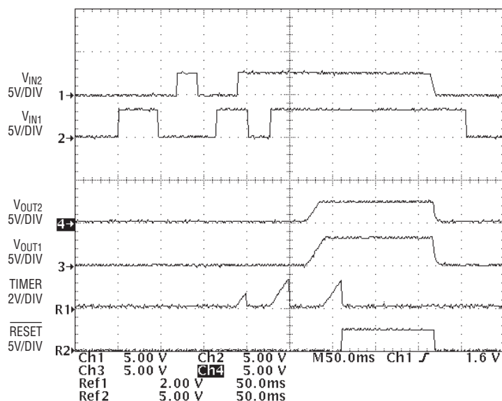
Figure 16. Ramping 3.3V and 2.5V Up and Down Together
