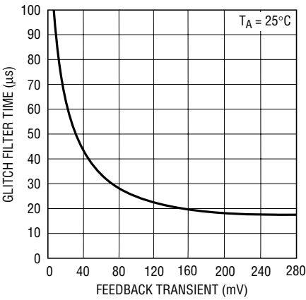
Glitch Filter Time vs Feedback Transient
