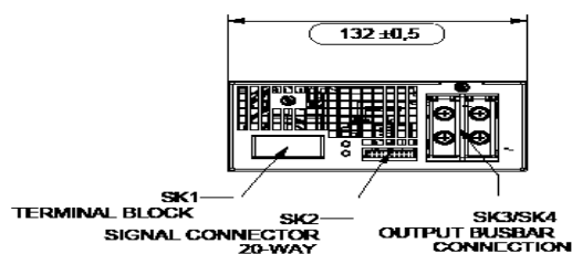
PSU Front View (24V & 48V UNITS)
