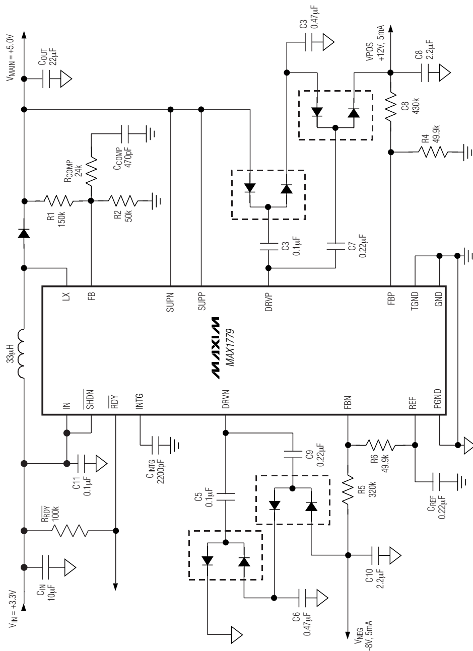
Figure 5. Typical Operating Circuit ( L = 33\mu H )
