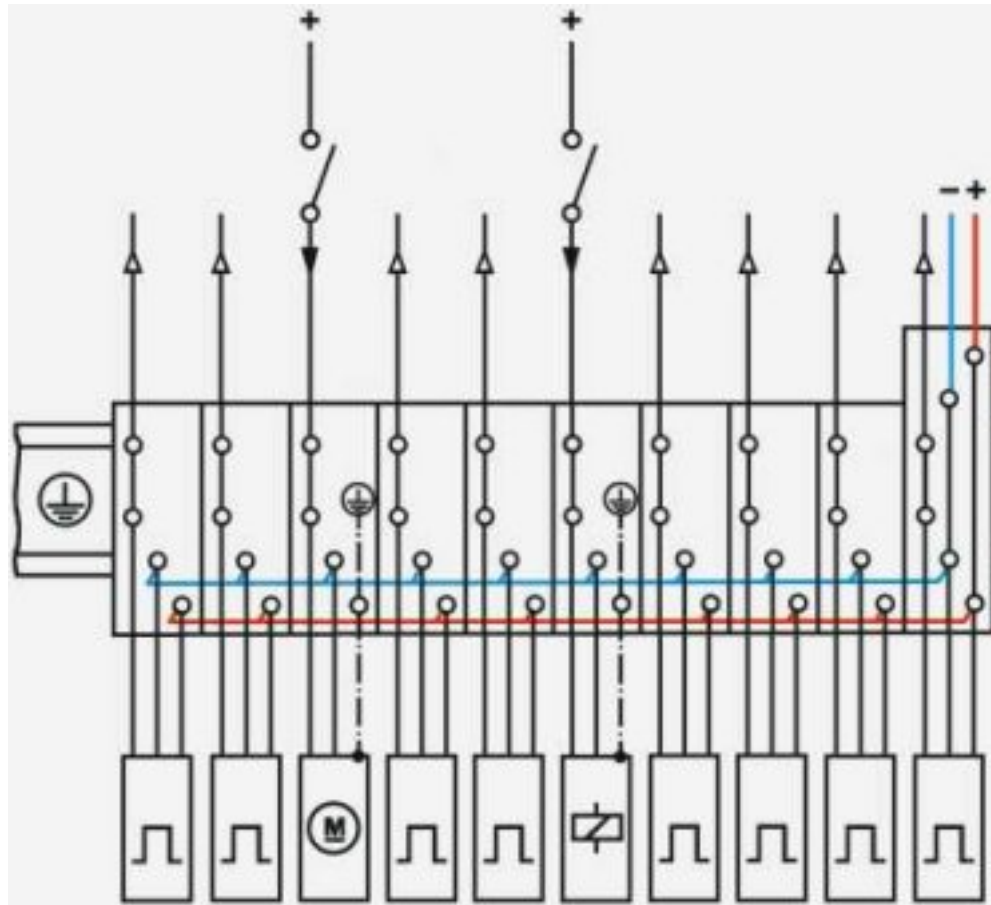
Circuit diagram
