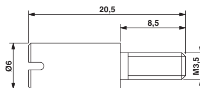
Dimensioned drawing
