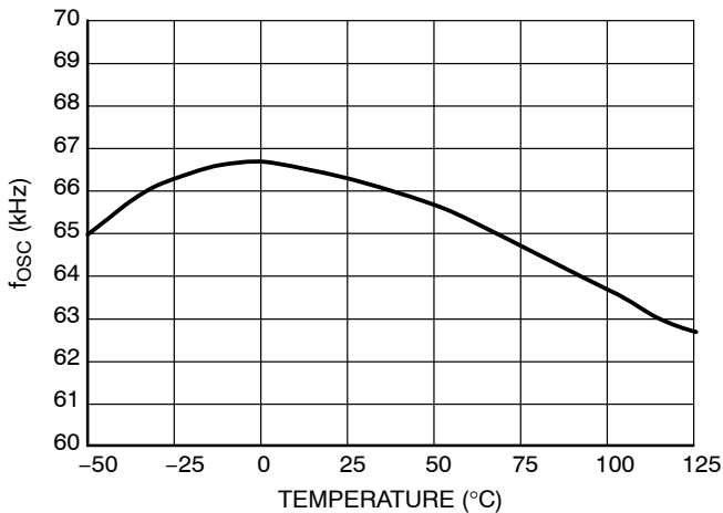
Figure 13. Oscillator Frequency f_{\text{osc}} for the 65 kHz version
