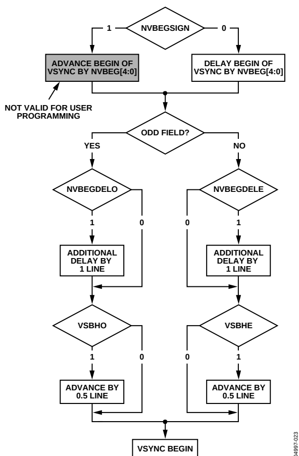
Figure 23. NTSC Vsync Begin
