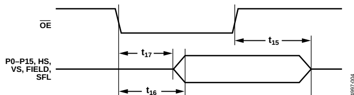
Figure 4. OE Timing
