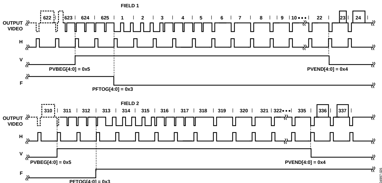
Figure 26. PAL Default (BT.656). The Polarity of H, V, and F is Embedded in the Data.
