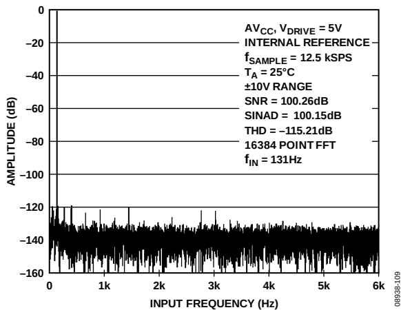
Figure 10. FFT Over Sampling by 16, \pm 10 V Range
