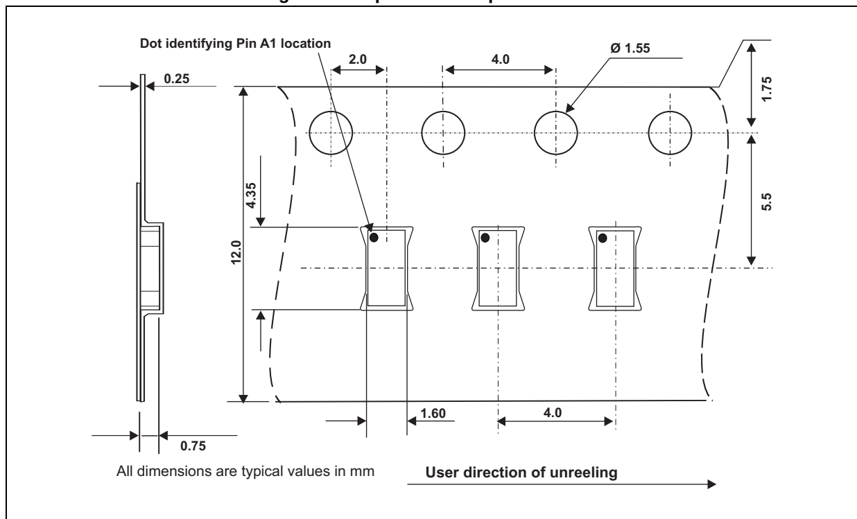
Figure 20. Tape and reel specifications
