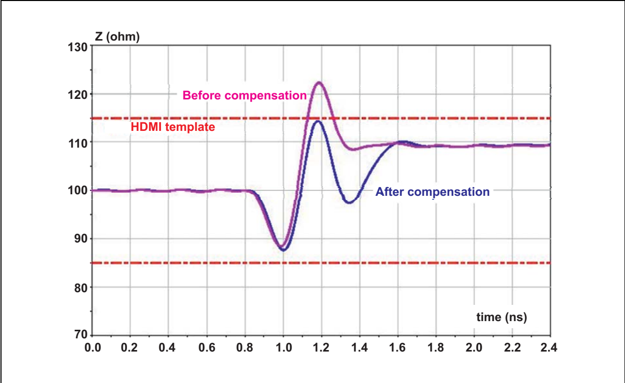
Figure 13. TDR
