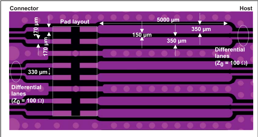
Figure 15. PCB layout recommendations
