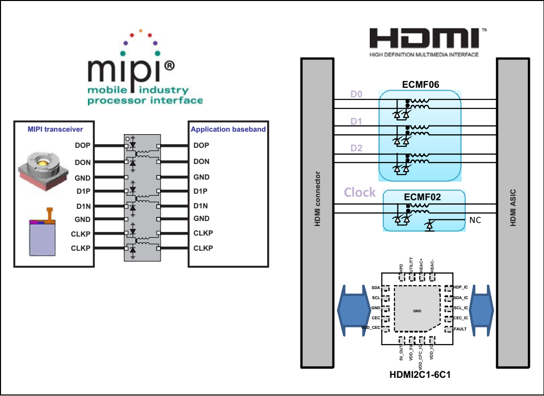
Figure 14. HDMI schematic
