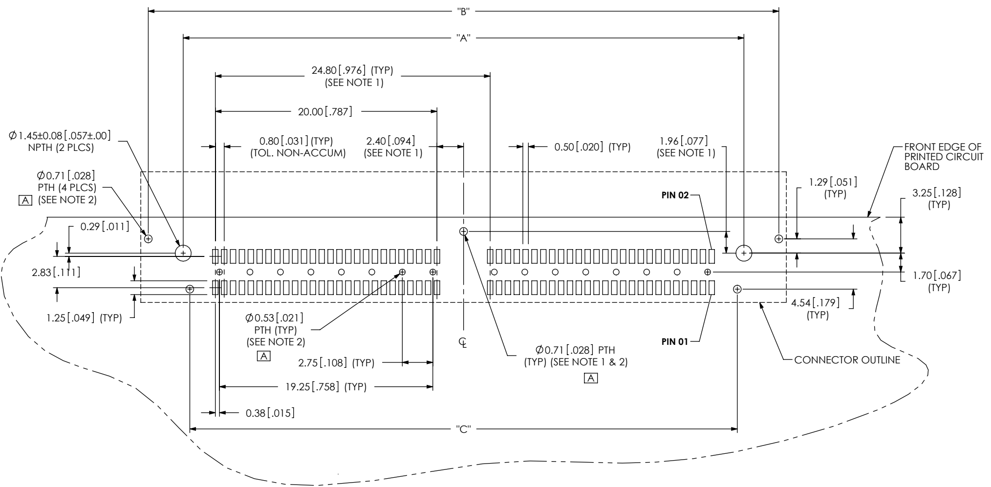
QRM8-052-XX-X-RA-GP-TR (ALL DIMENSIONS ARE SYMMETRIC ABOUT THE CENTERLINE)
