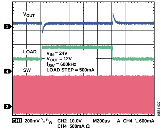
Figure 37. Load Transient Response, V_{IN} = 24\text{V} , V_{OUT} = 12\text{V} , f_{SW} = 600\text{kHz} , Load Step = 500 mA
