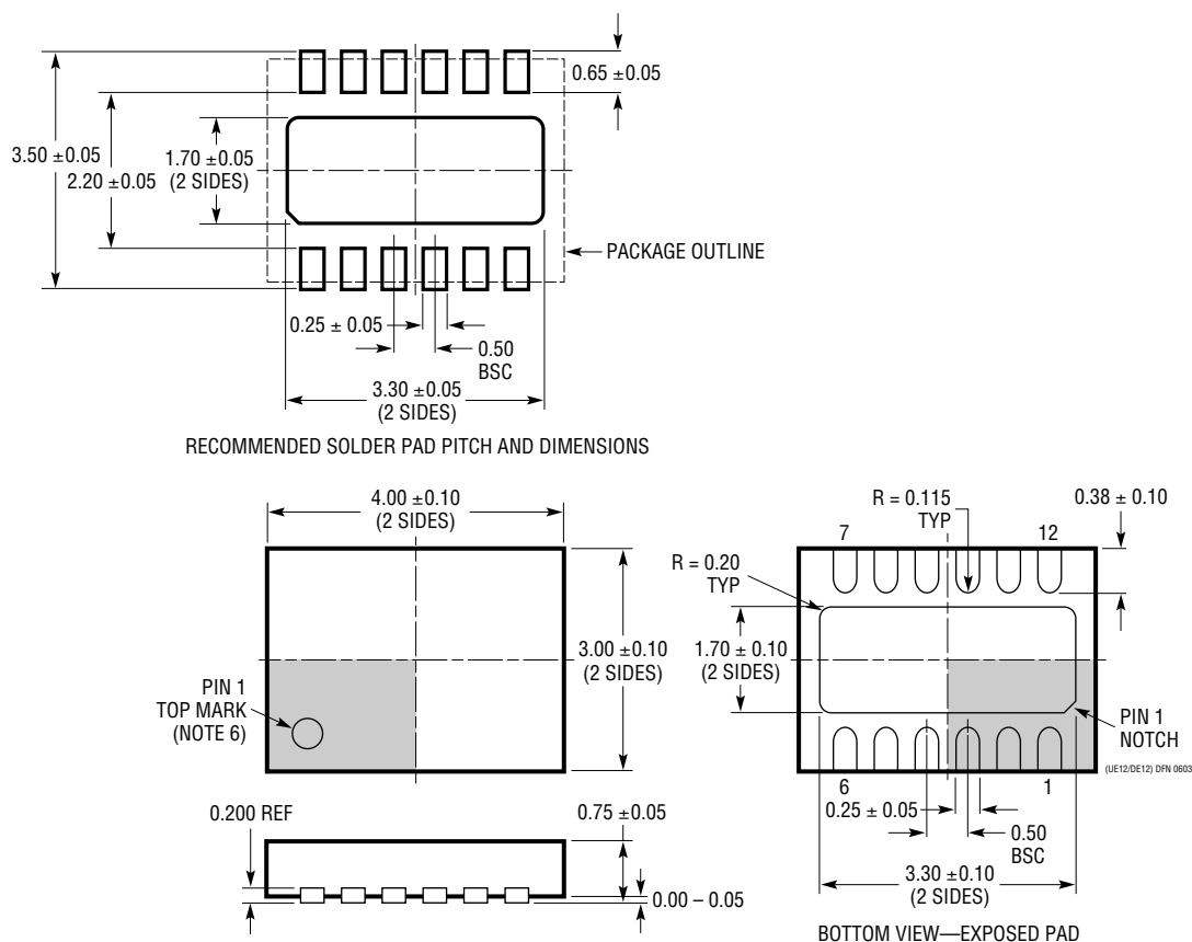
DE/UE Package 12-Lead Plastic DFN (4mm × 3mm) (Reference LTC DWG # 05-08-1695)
