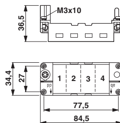
Dimensioned drawing
