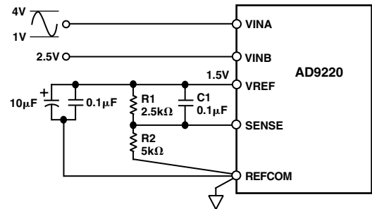
Figure 23. Resistor Programmable Reference—3 V p-p Input Span, V_{CM} = 2.5 V
