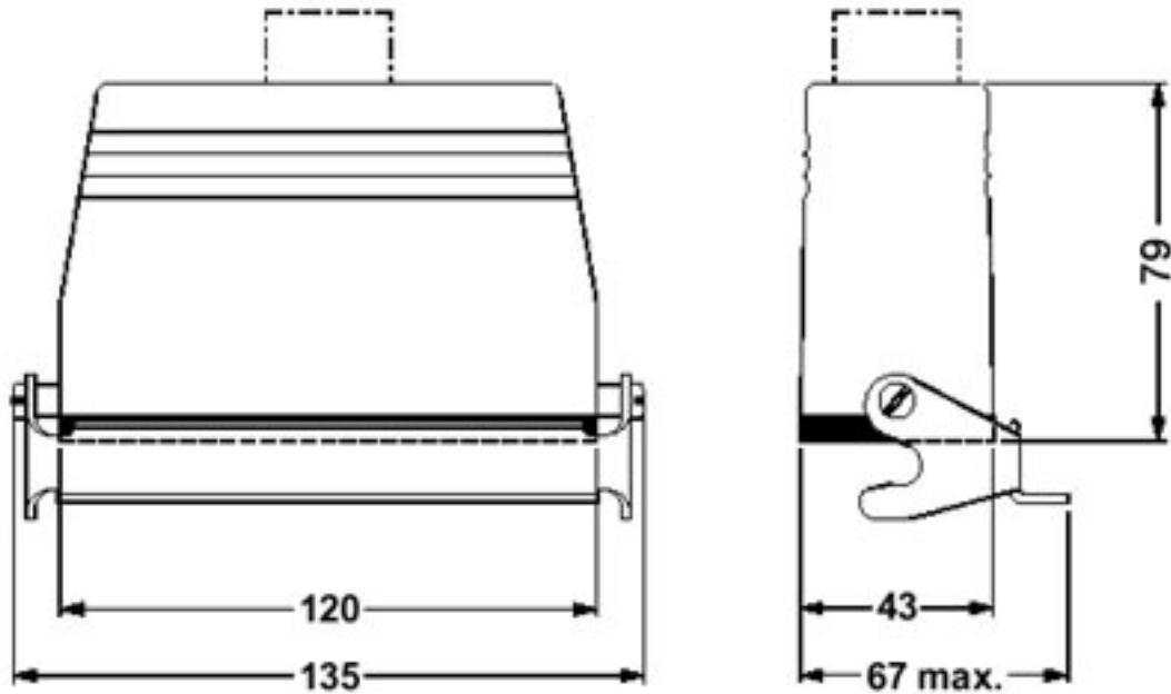
Dimensioned drawing
