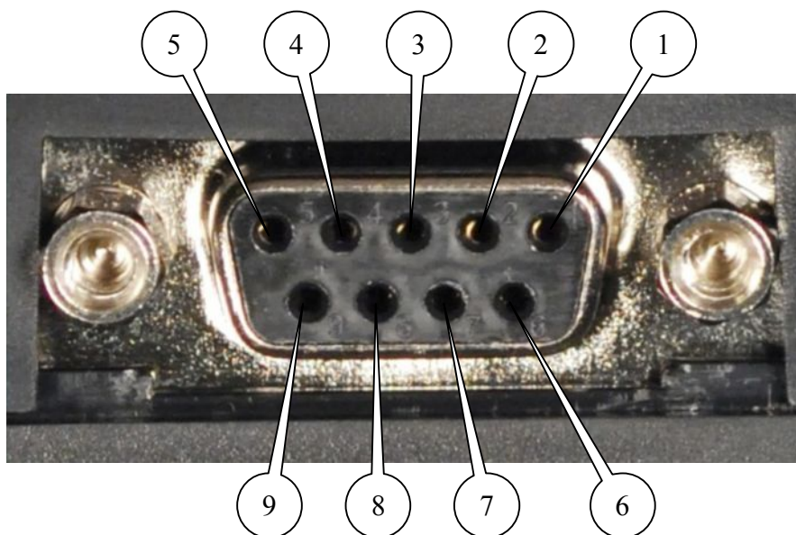
Fig.2.5.1 Connector DB9
