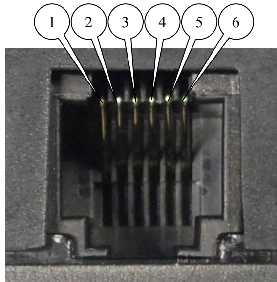
Fig.2.5.3 Connector RJ11
