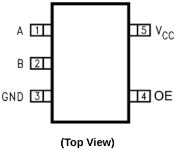
Pad Assignment for MicroPak
