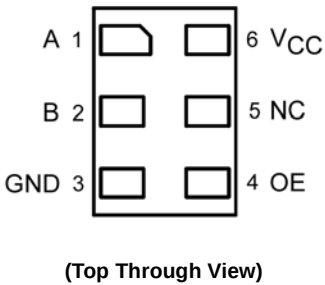
Pad Assignment for MicroPak
