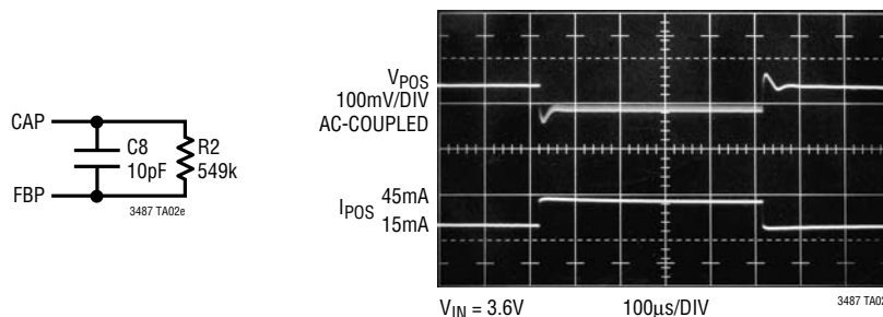
VPOS Load Step Response (with Phase Lead Capacitor)
