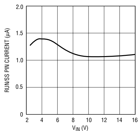
RUN/SS Pin Current vs VIN in Shutdown
