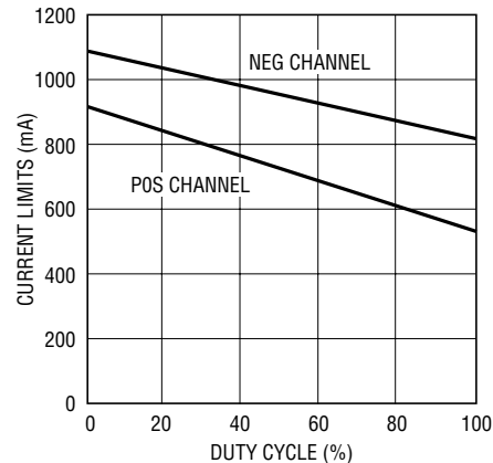
Switch Current Limits vs Duty Cycle
