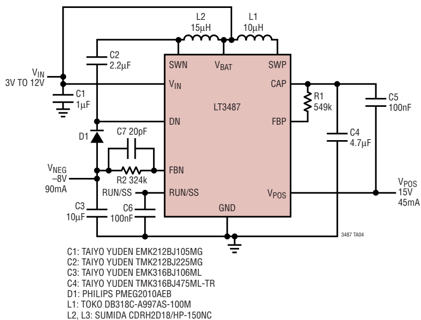
+15V and -8V Boost and Charge Pump CCD Bias
