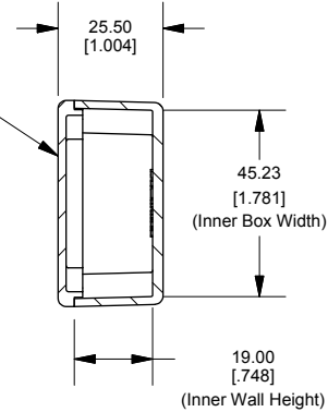
SECTION A-A End View of Assembly
