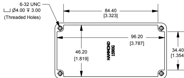
Top View Looking Inside Box
