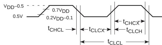
Figure 59. Clock Signal Waveform for I DD Tests in Active and Idle Modes t_{CLCH} = t_{CHCL} = 5\text{ns}
