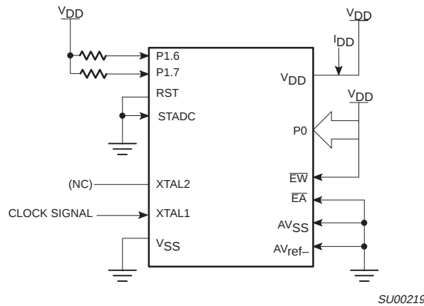
Figure 58. I DD Test Condition, Idle Mode All other pins are disconnected 2
