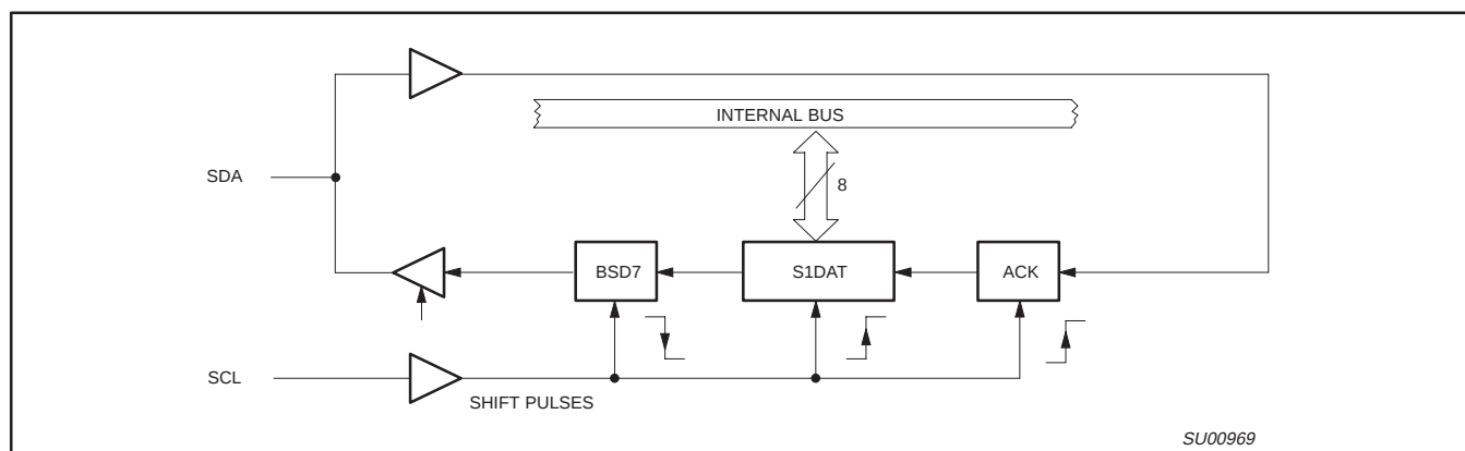
Figure 37. Serial Input/Output Configuration
