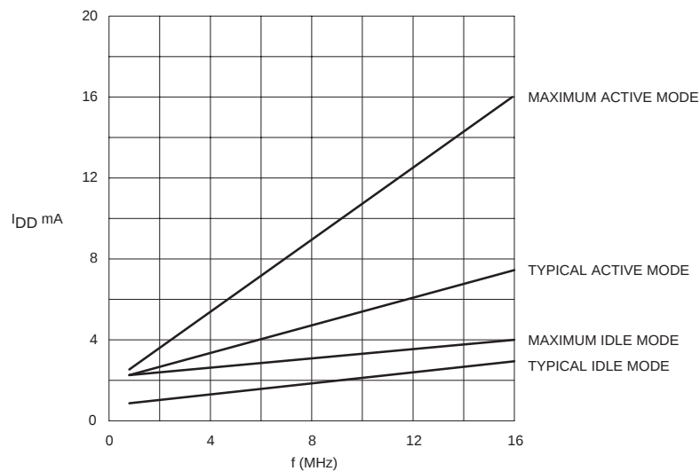
Figure 56. 16MHz Version Supply Current ( I_{DD} ) as a Function of Frequency at XTAL1 ( f_{osc} )
