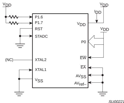
Figure 60. I DD Test Condition, Power Down Mode All other pins are disconnected. V DD = 2V to 5.5V 3
