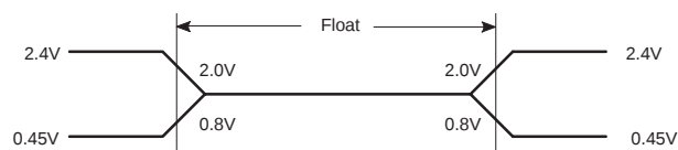
Figure 53. AC Testing Input/Output
