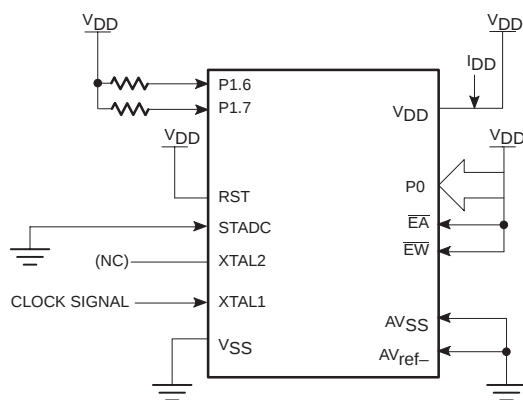
Figure 57. I_{DD} Test Condition, Active Mode All other pins are disconnected 1
