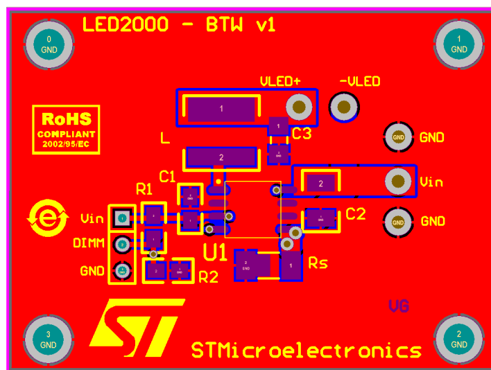
Figure 22. PCB layout (component side) SO8 package
