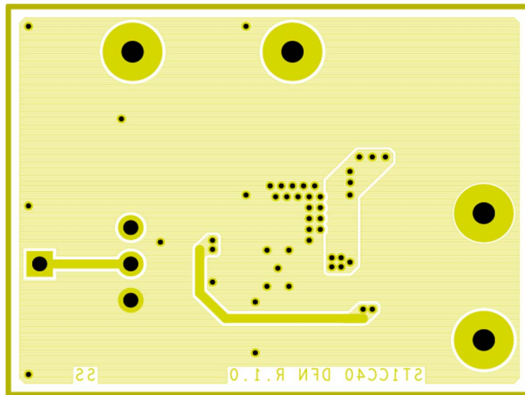
Figure 21. PCB layout (bottom side) VFQFPN package
