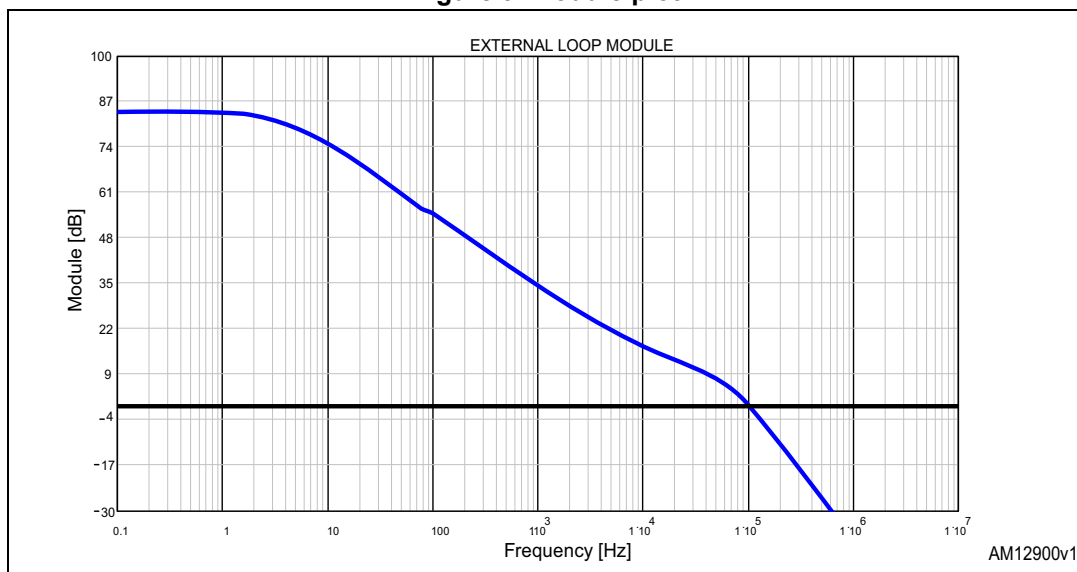
Figure 9. Module plot
