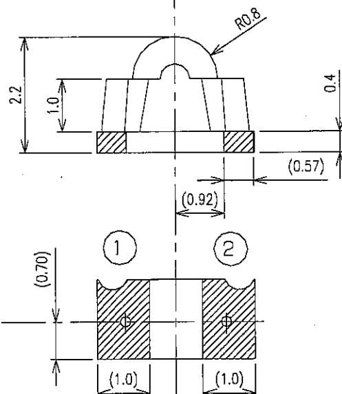
The pattern example from the view point of PCB (Top view)
