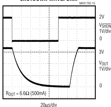
SHUTDOWN WAVEFORM
