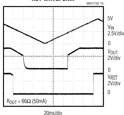
\overline{\text{RST}} WAVEFORM
