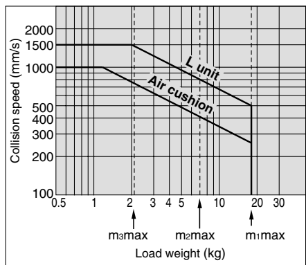
MY1C16 Horizontal collision: P = 0.5 MPa
