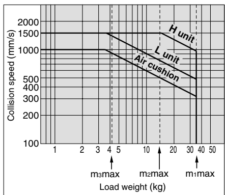
MY1C25 Horizontal collision: P = 0.5 MPa
