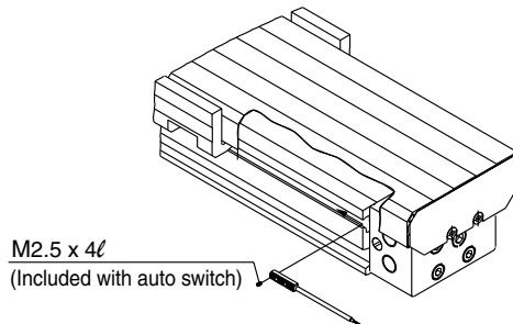
Fig. (2) Auto switch mounting
