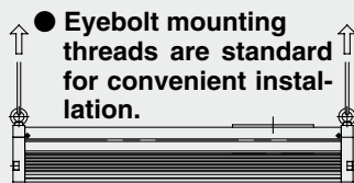
Using eyebolts
