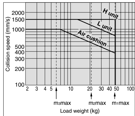
MY1C32 Horizontal collision: P = 0.5 MPa
