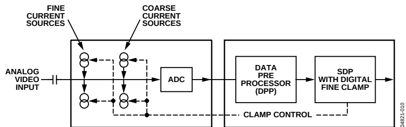
Figure 10. Clamping Overview
