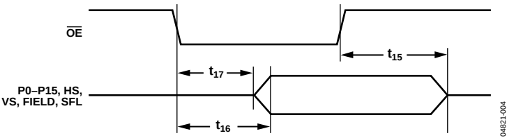
Figure 4. OE Timing
