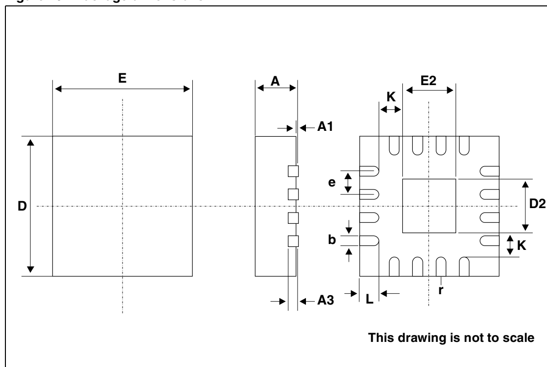
Figure 29. Package dimensions
