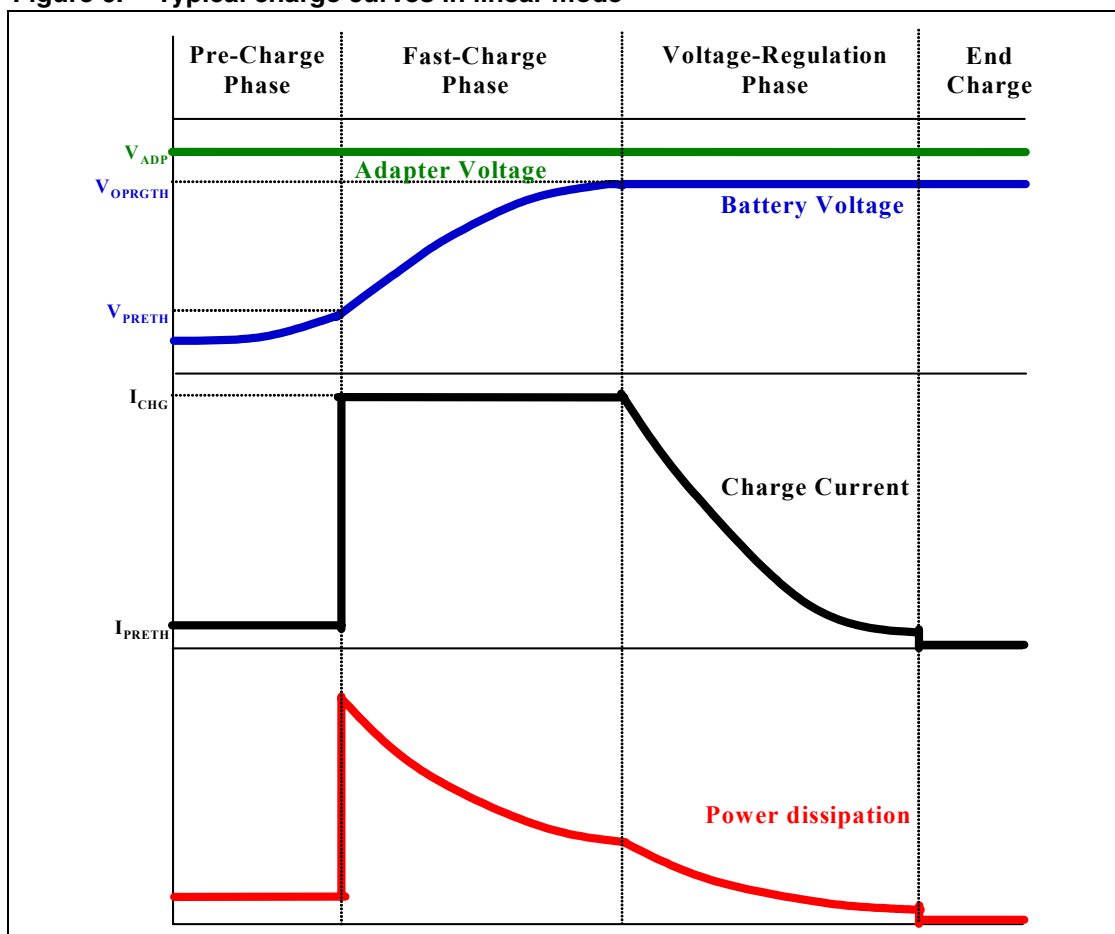
Figure 6. Typical charge curves in linear mode
