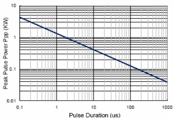
FIG 5. Non-Repetitive Peak Pulse Power vs. Pulse Time
