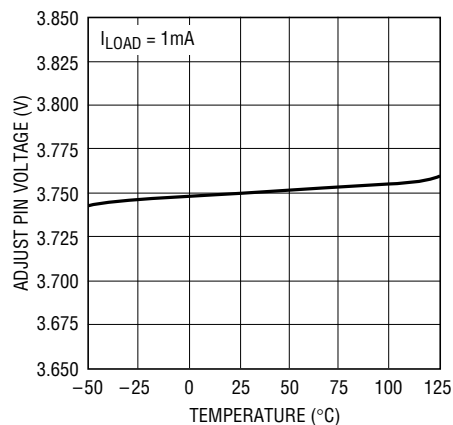
LT1529 Adjust Pin Voltage
