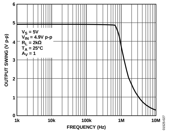
Figure 27. Closed-Loop Output Voltage Swing vs. Frequency
