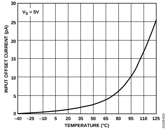
Figure 15. Input Offset Current vs. Temperature
