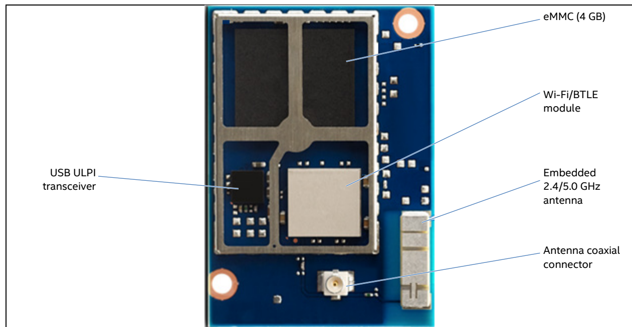
Figure 2 Edison top view
