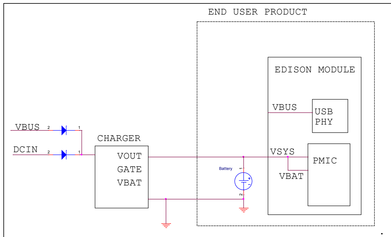
Figure 5 Example Edison lithium-polymer battery direct attach
