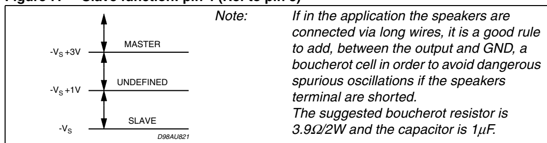
Figure 7. Slave function: pin 4 (Ref to pin 8)
