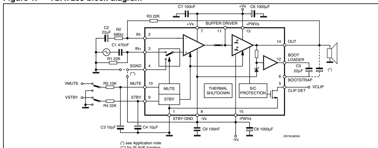
Figure 1. TDA7293 block diagram
