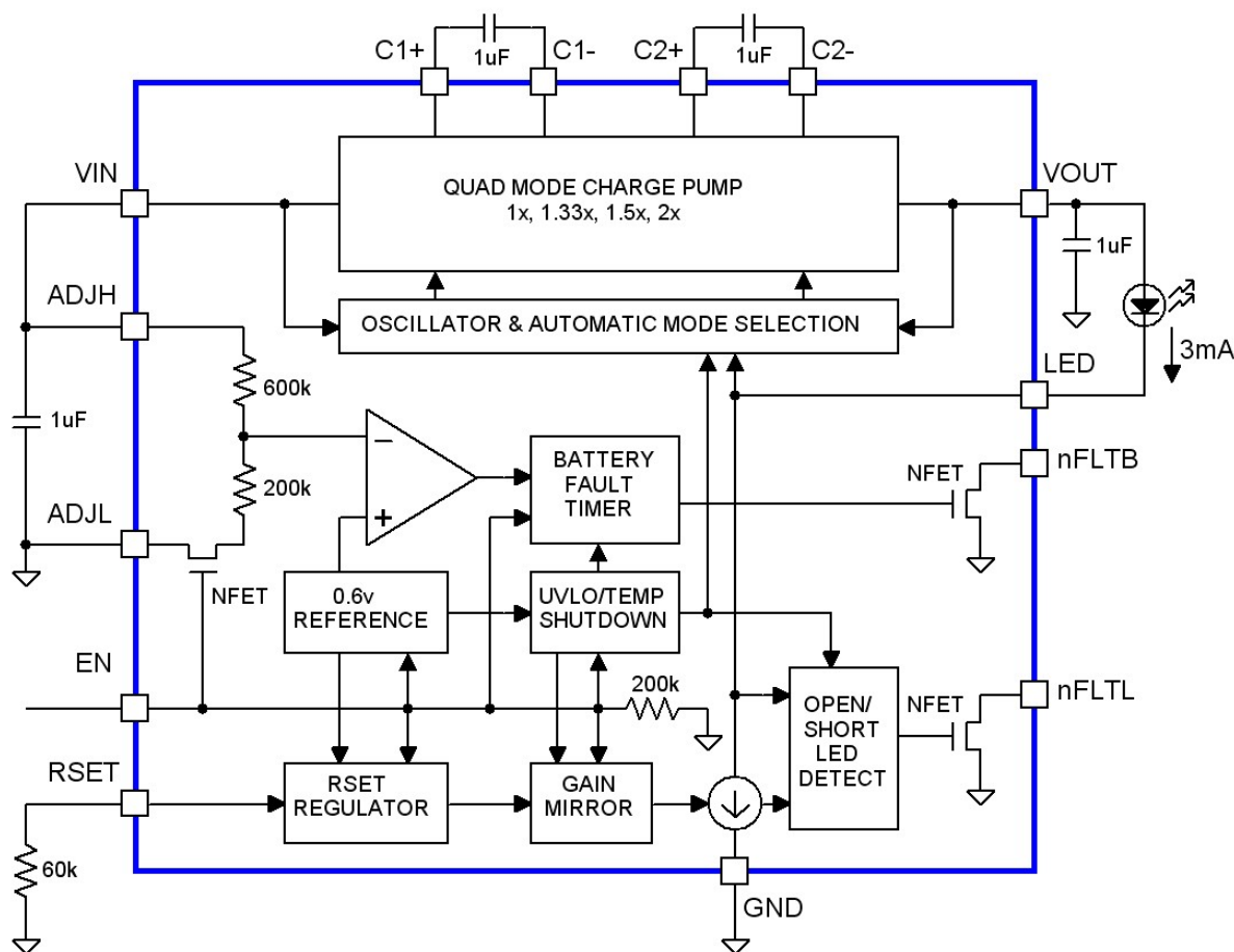
Figure 24. CAT3661 Functional Block Diagram
