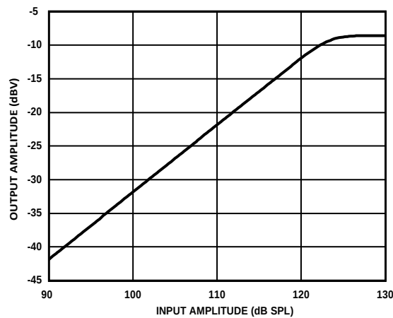
Figure 7. Linearity
