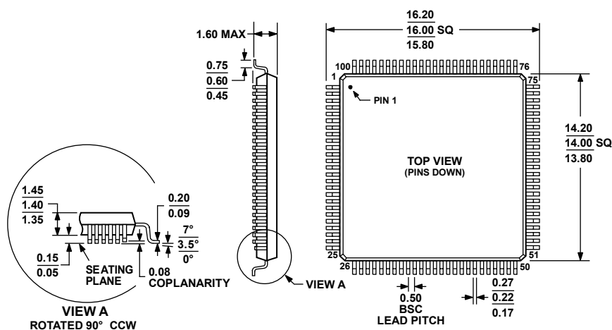
Figure 36. 100-Lead Low Profile Quad Flat Package [LQFP] (ST-100) Dimensions shown in millimeters
