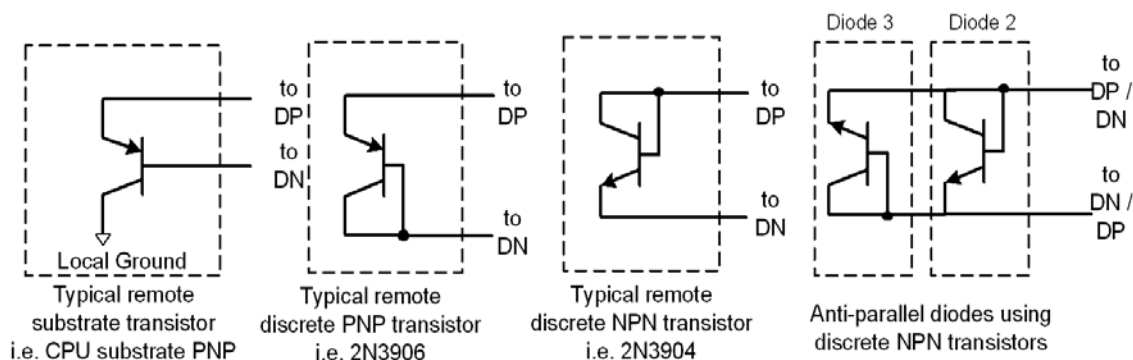
Figure 6.6 Diode Connections
