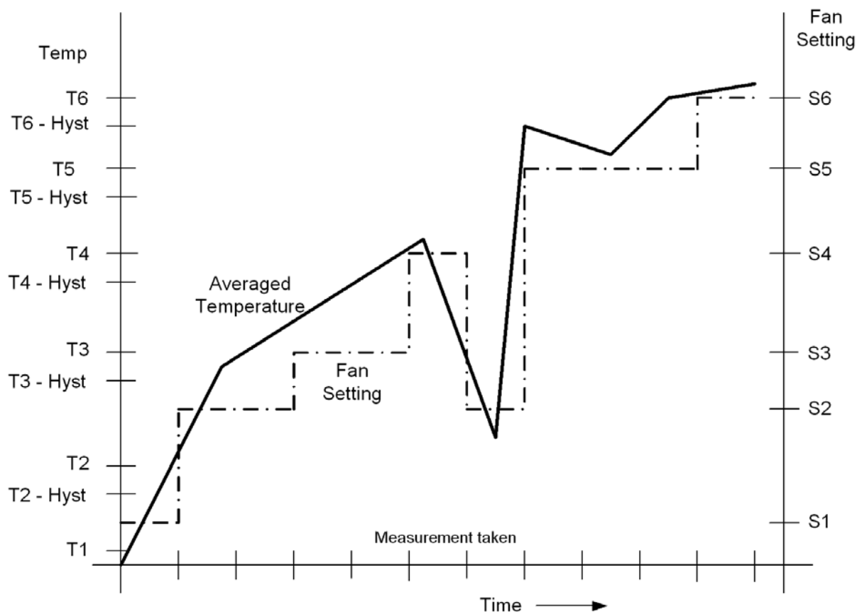
Figure 6.3 Fan Control Look-Up Table Example
