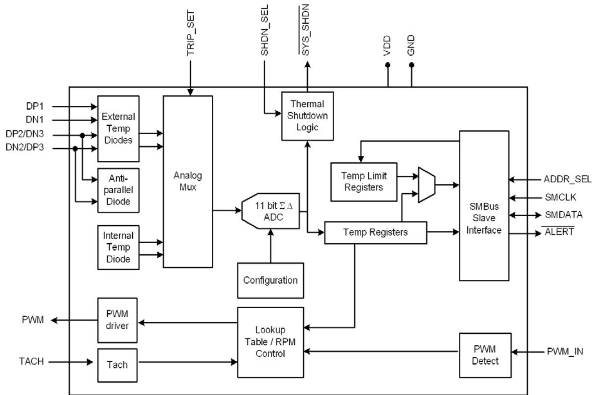
Figure 1.1 EMC2113 Block Diagram
