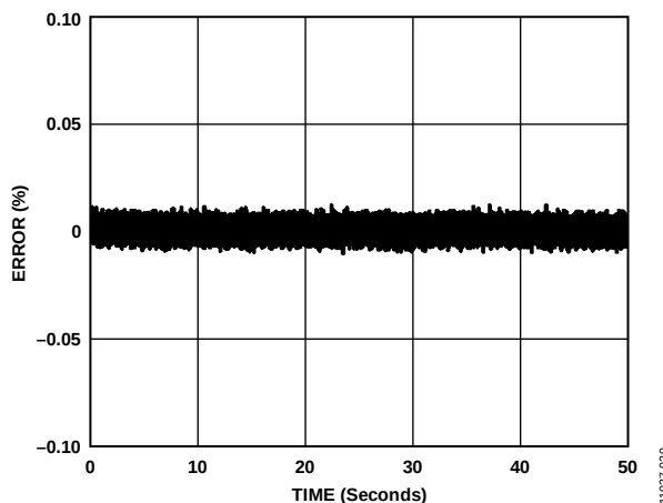
Figure 19. Internal Reference Settling Time (Extended) (AVDD1 = 5 V, AVDD2 = 5 V, IOVDD = 3.3 V)
