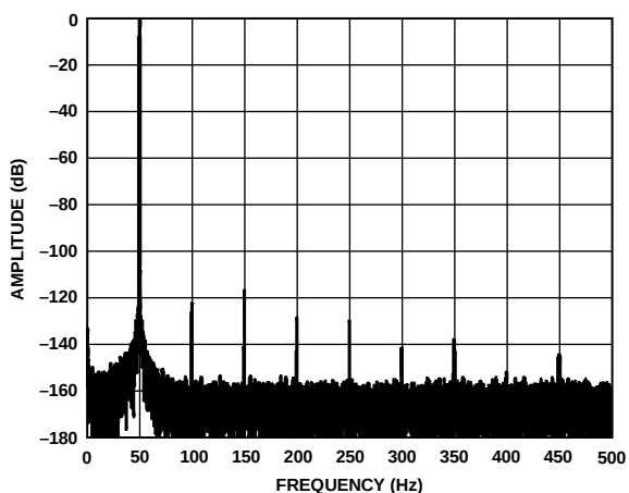
Figure 13. 50 Hz Input Tone, -0.5 dBFS Input FFT (AVDD1 = 5 V, AVDD2 = 5 V, IOVDD = 3.3 V, V REF = 2.5 V, Output Data Rate = 1 kSPS)
