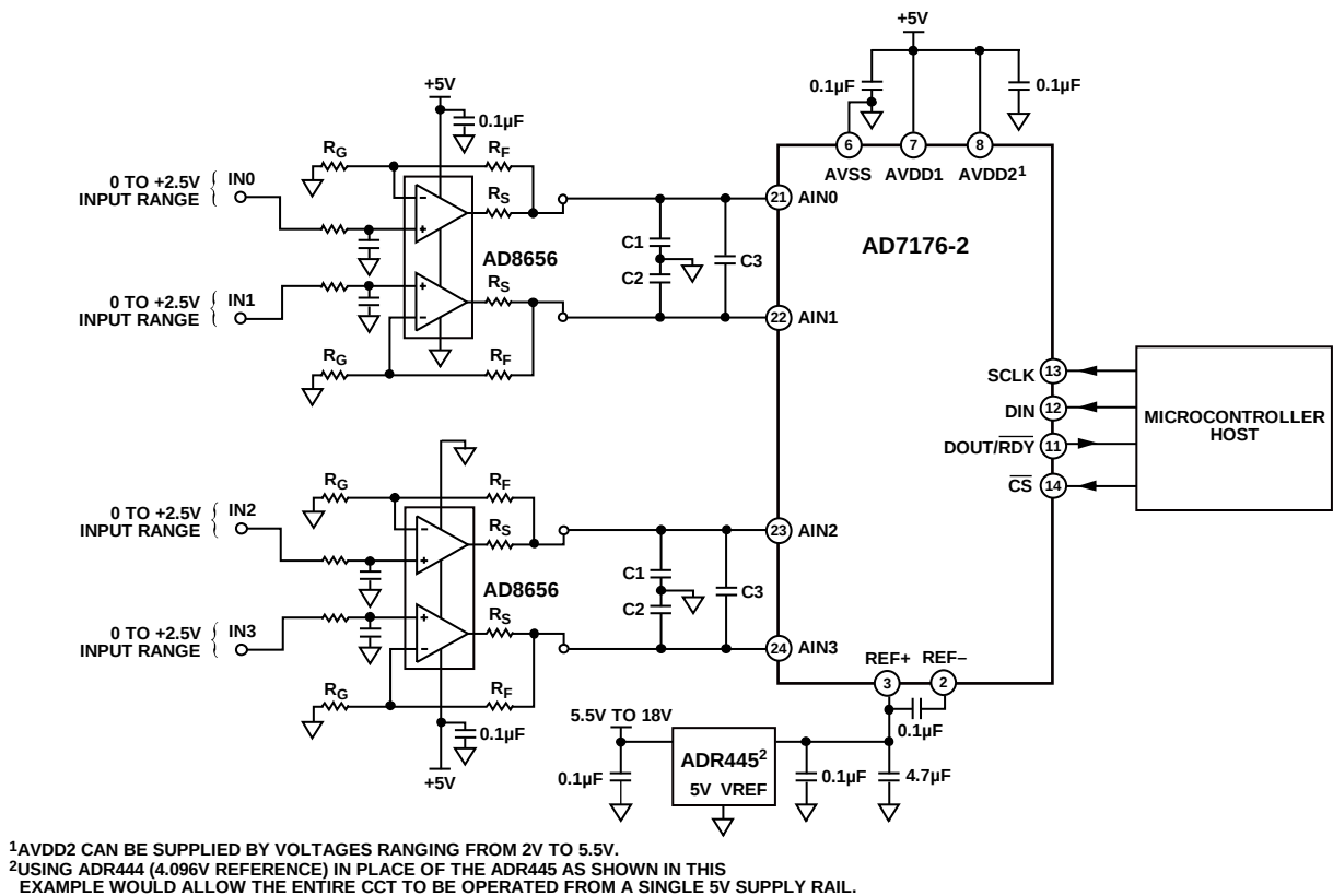
Figure 31. Dual AD8656 Amplifiers Driving the AD7176-2
