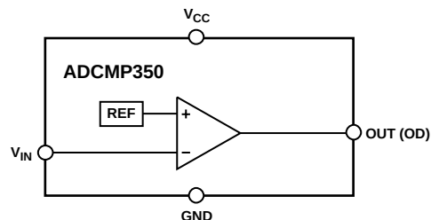
Figure 1. ADCMP350 Functional Block Diagram
