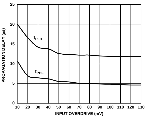
Figure 17. Propagation Delay vs. Input Overdrive ( V_{CC} = 3.3 V, Push-Pull Only)
