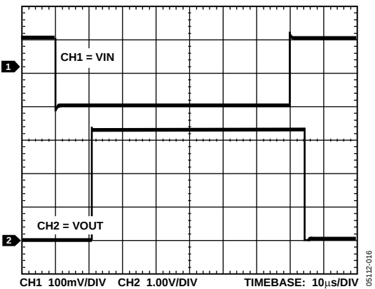
Figure 19. Propagation Delay Timing, 100 mV Overdrive
