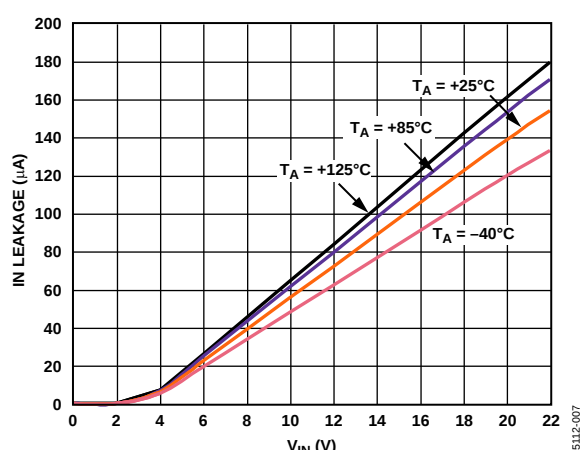
Figure 8. Input Leakage vs. Input Voltage ( V_{IN} )
