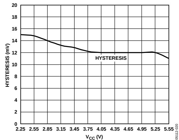
Figure 12. V_{IN} Trip Hysteresis vs. V_{CC}
