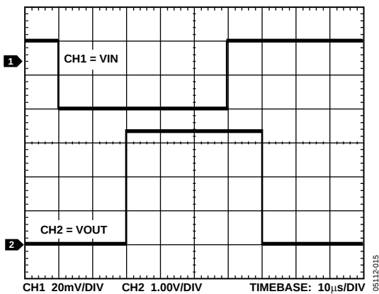
Figure 18. Propagation Delay Timing, 10 mV Overdrive
