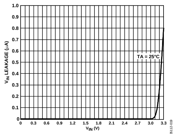
Figure 9. V_{IN} Leakage Current vs. V_{IN} Voltage ( V_{CC} = 3.8 V)
