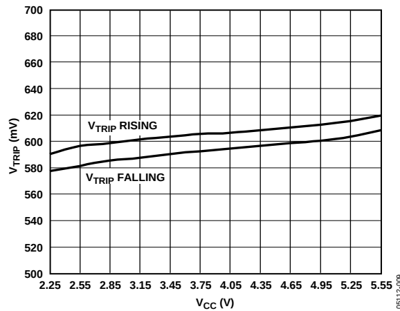
Figure 11. V_{IN} Trip Threshold vs. V_{CC}
