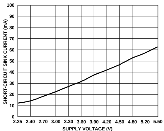
Figure 16. Short-Circuit Sink Current vs. Supply Voltage ( V_{CC} = 3.3 V, Push-Pull Only)
