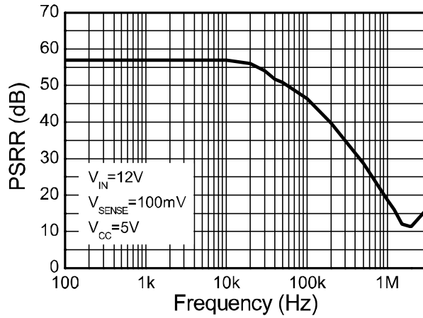
Supply Rejection
