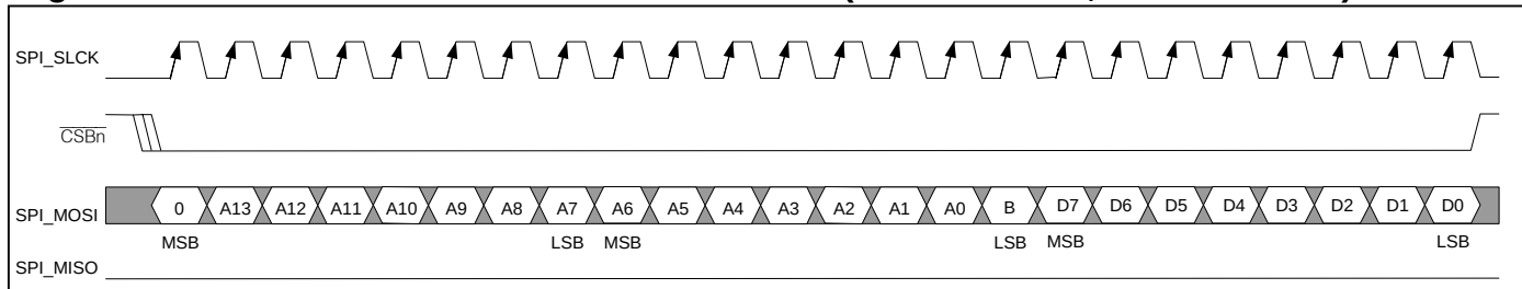
Figure 8-5. SPI Serial Port Access for Write Mode (SPI_CPOL = 0, SPI_CPHA = 0)
