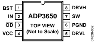
Figure 4. SOIC_N Pin Configuration
