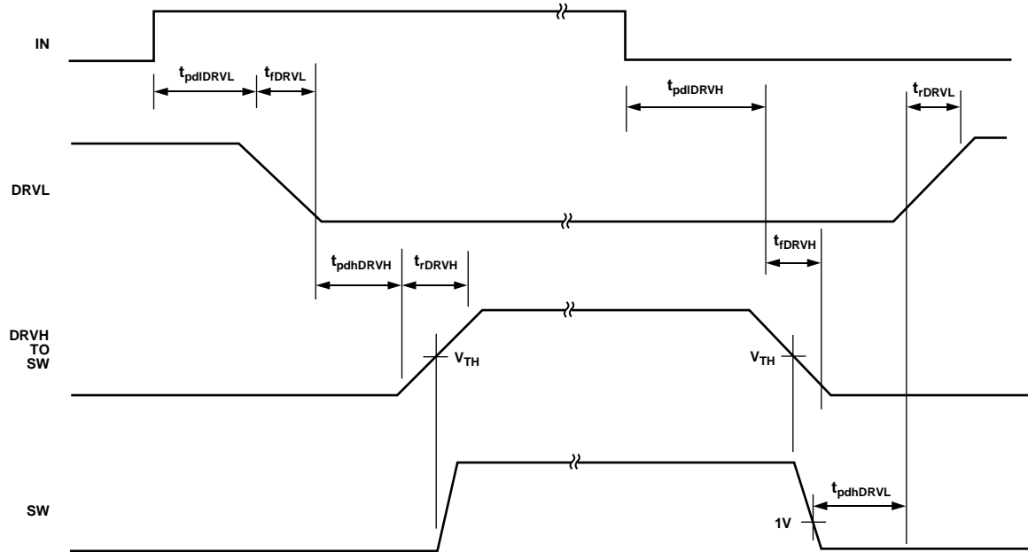
Figure 3. Timing Diagram
