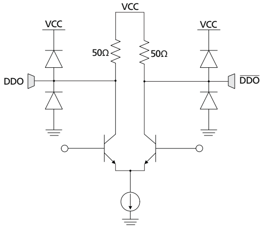
Figure 3-6: High-speed Outputs (DDO1/RCO, DDO0)
