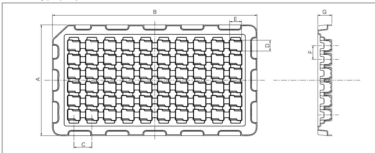
Blister Tray Dimention
