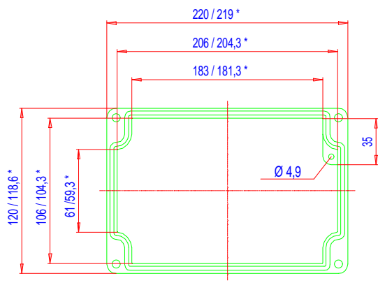
Deckel
