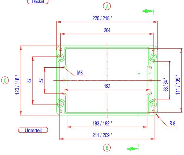
Deckel
