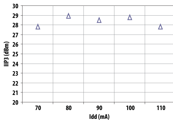
Figure 12. IIP3 vs Idd at 4.8 V Tuned for Optimum IIP3 and Fmin at 900 MHz
