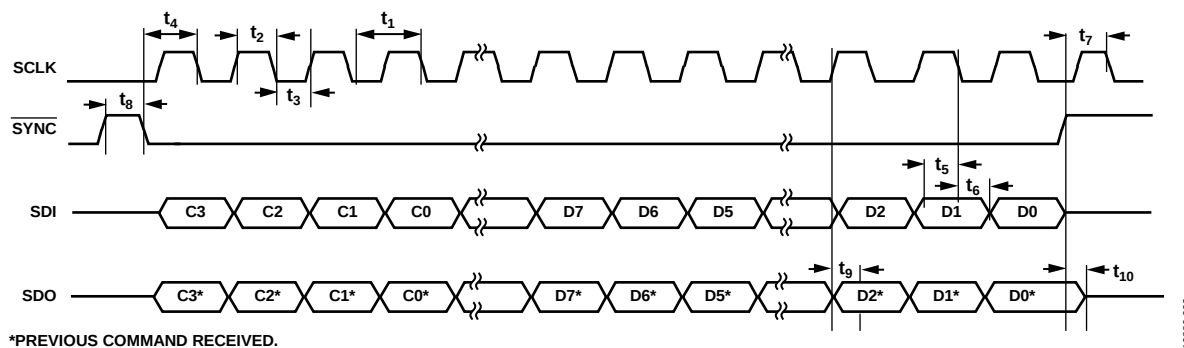
Figure 3. SPI Serial Interface Timing Diagram, CPOL = 0, CPHA = 1
