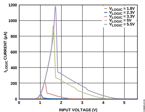
Figure 19. I_{\text{LOGIC}} Current vs. Digital Input Voltage
