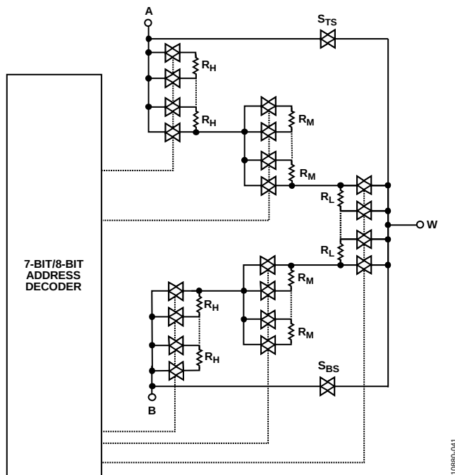
Figure 41. AD5122/AD5142 Simplified RDAC Circuit
