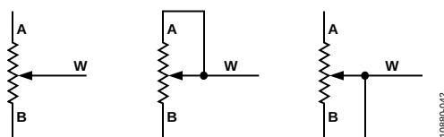
Figure 42. Rheostat Mode Configuration
