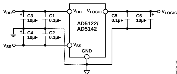
Figure 45. Power Supply Bypassing
