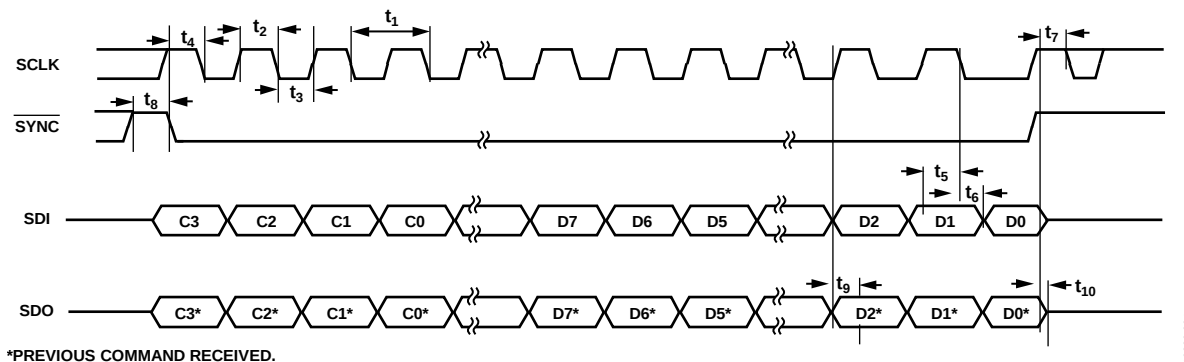
Figure 4. SPI Serial Interface Timing Diagram, CPOL = 1, CPHA = 0
