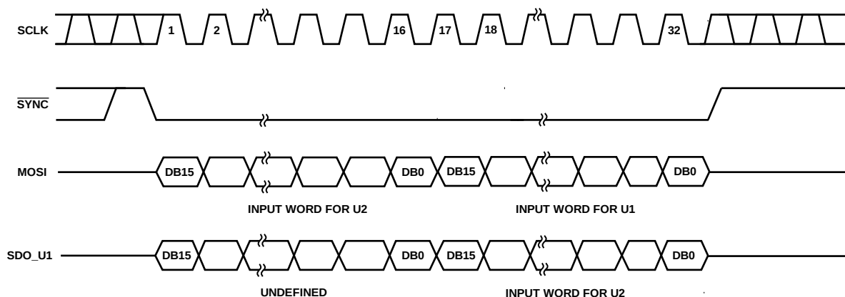
Figure 40. Daisy-Chain Diagram
