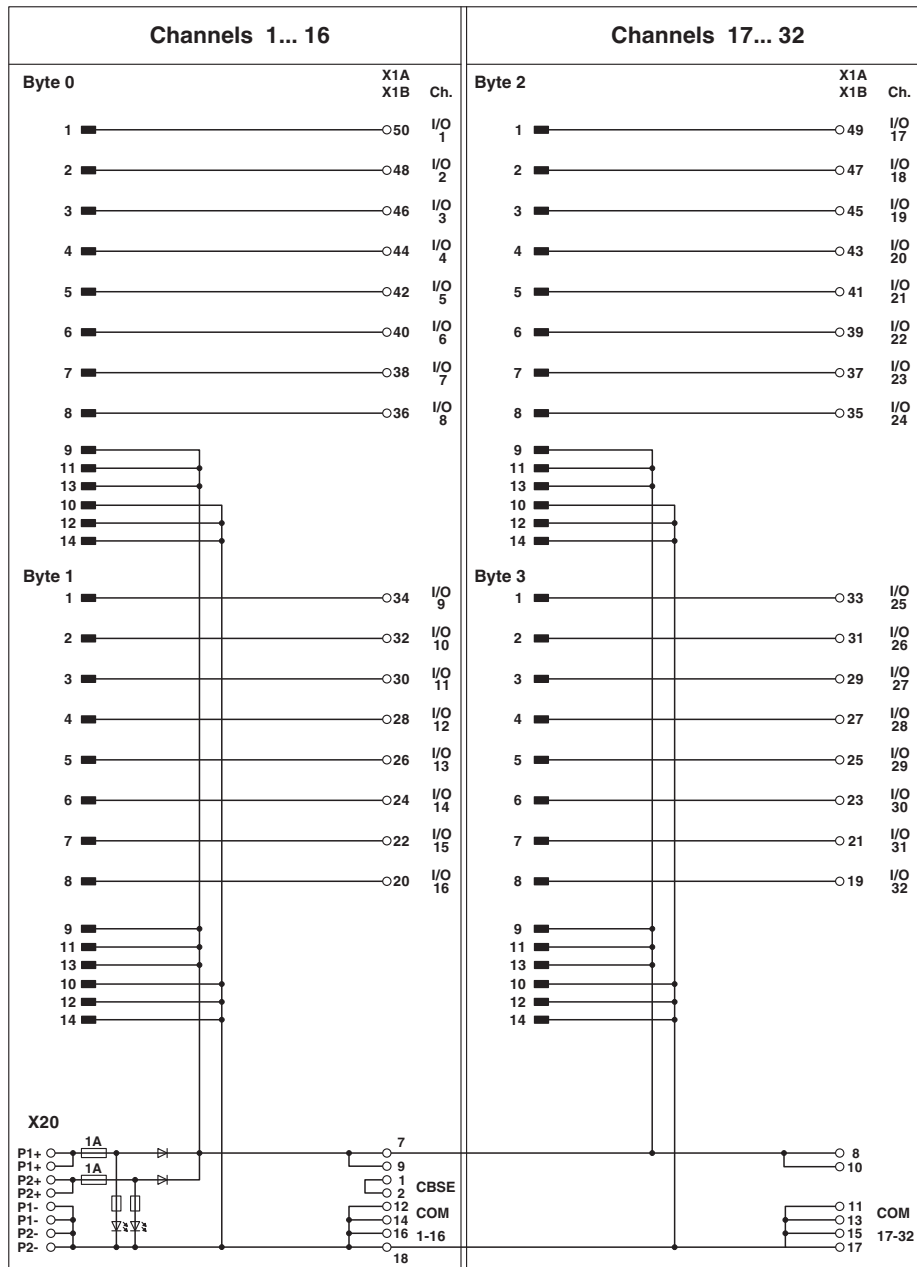
Circuit diagram
