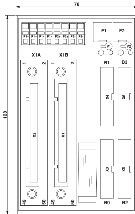
Dimensioned drawing
