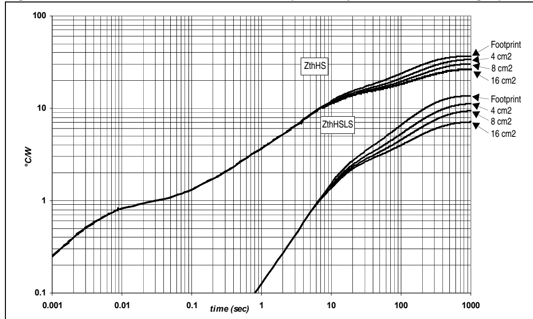
Figure 41. MultiPowerSO-30 HSD thermal impedance junction ambient single pulse
