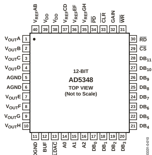
Figure 10. AD5348 Pin Configuration—LFCSP
