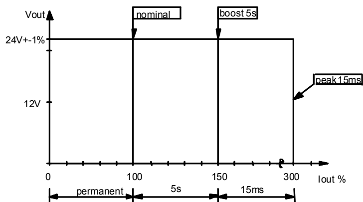
Fig 1 Current capability
