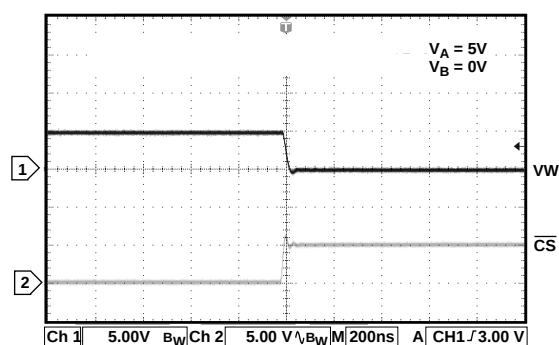
Figure 26. Midscale Glitch, Code 0x80 to Code 0x7F
